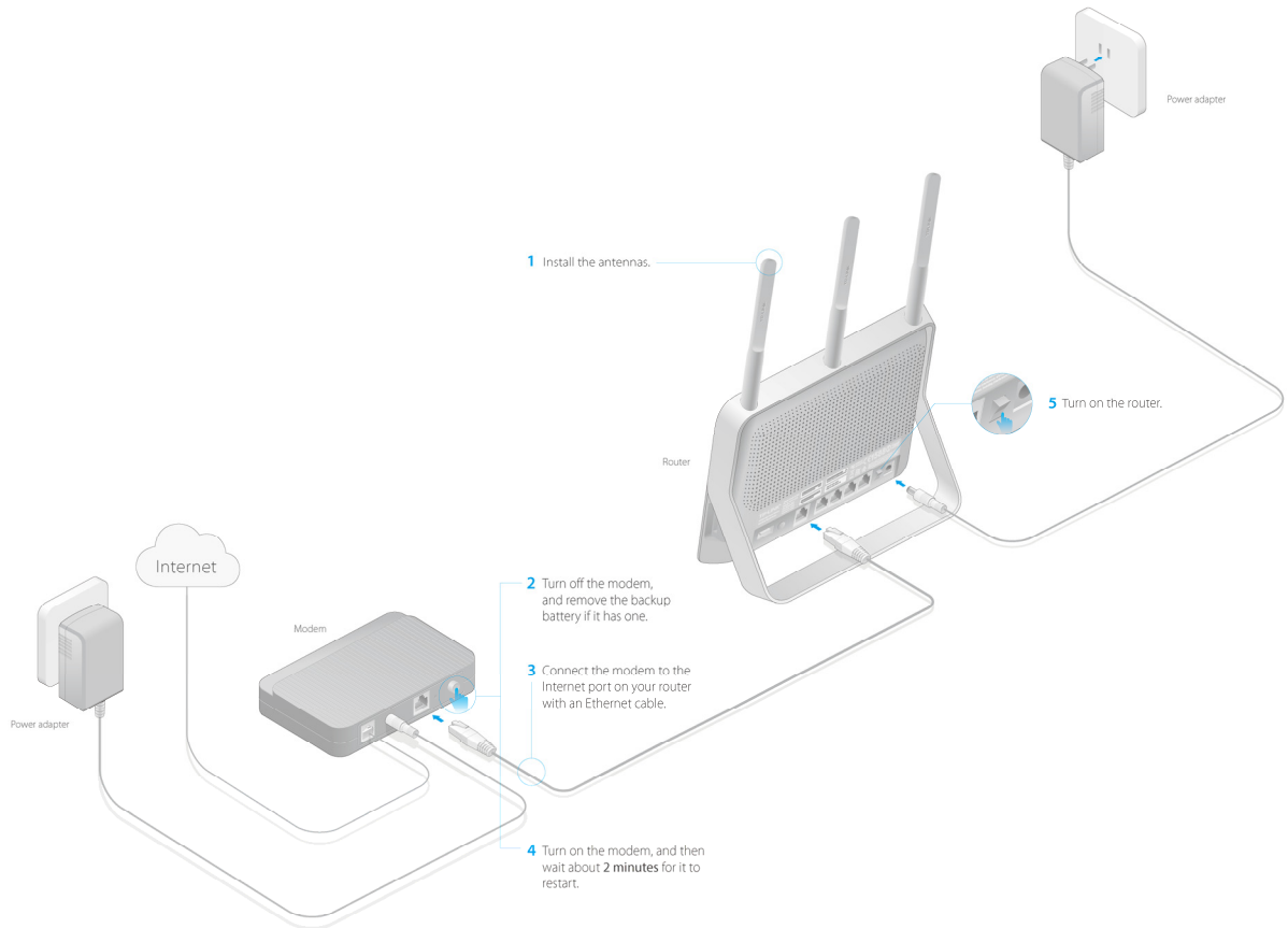
Figure 2-1 Hardware Installation
